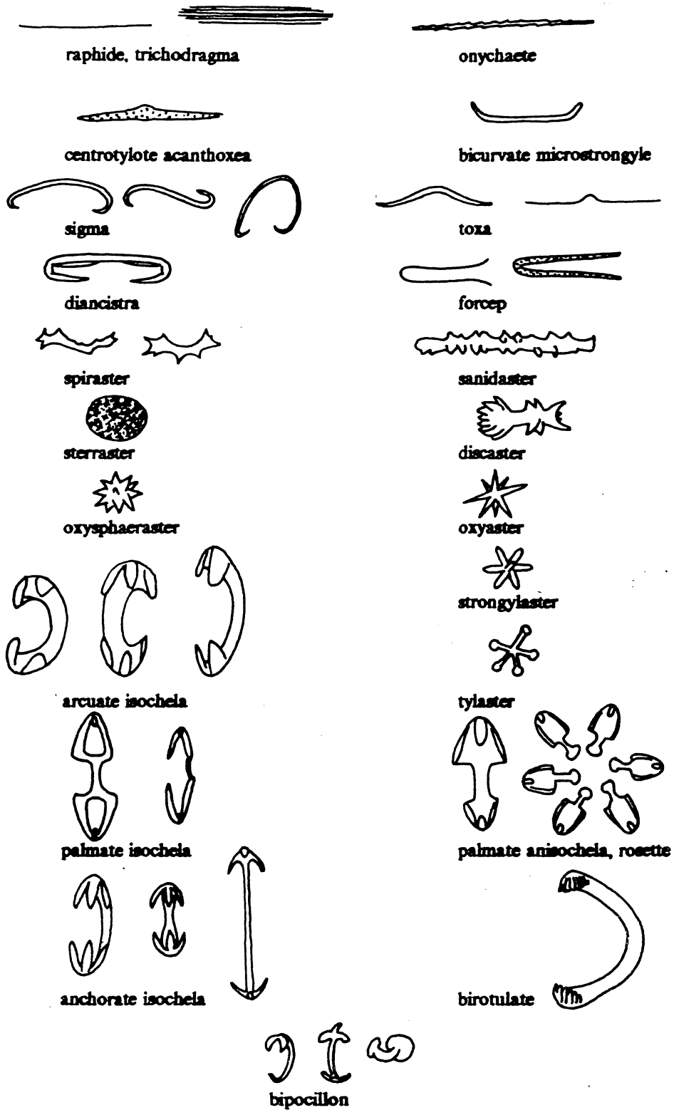
Figure 2. Demospongiae microscleres
