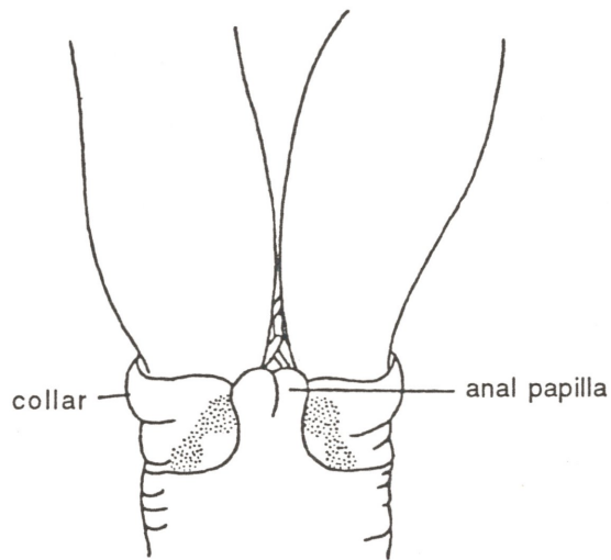
lophophoral end of Phoronopsis showing base of lophophore ridge, anus and collar.
