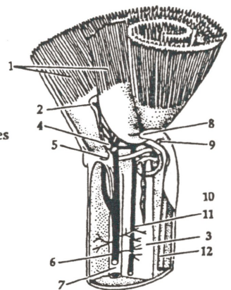
Schematic diagram of major internal organs in the lophophoral end of phoronid. (from Brusca & Brusca, 1990.)
