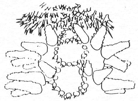
Figure 28. Ophiopholis bakeri .
