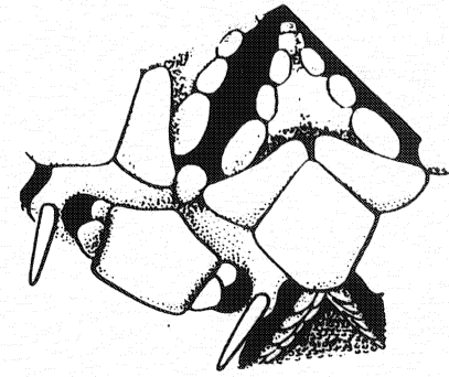
Figure 8. Amphichondrius granulatus .
