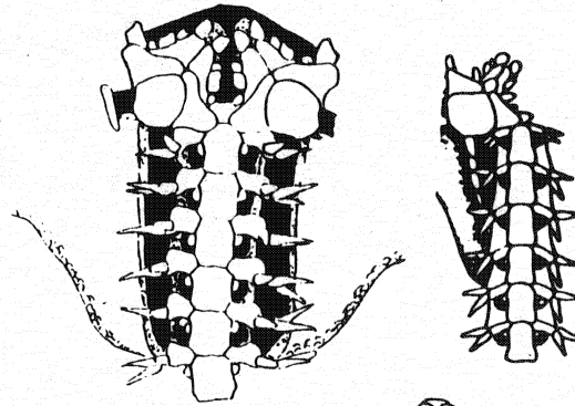
Figure 16. Amphioplus strongyloplax .
