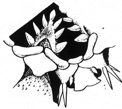
Figure 31. Ophiacantha normani .
