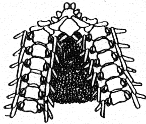
Figure 14. Amphiodia occidentalis .
