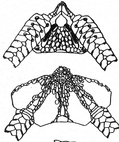
Figure 21. Ophiomusium jolliensis .
