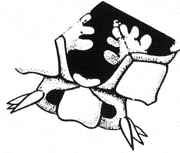
Figure 11. Amphiodia digitata .
