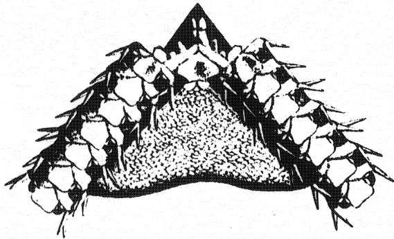
Figure 6. Amphiura diastata .
