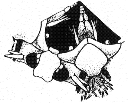
Figure 15. Amphiacantha amphacantha .
