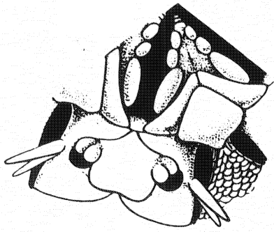
Figure 9. Amphipholis pugetana .
