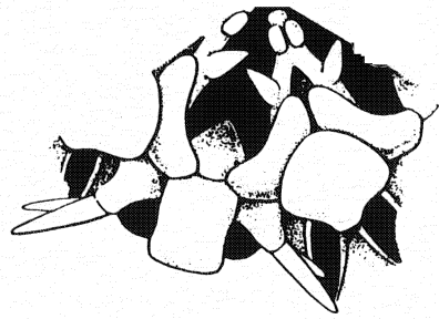
Figure 7. Amphiura arcystata .
