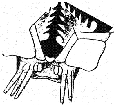
Figure 30. Ophiacantha diplasia .
