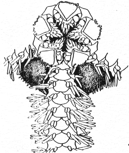
Figure 29. Ophiacantha phragma .
