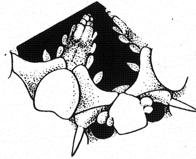
Figure 16. Amphioplus strongyloplax .
