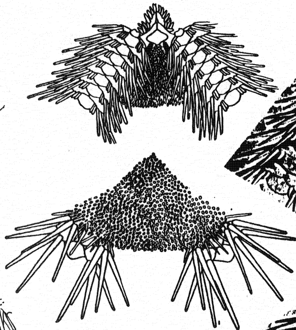
Figure 30. Ophiacantha diplasia .
