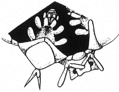
Figure 24. Ophiopsila californica .
