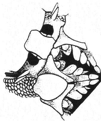
Figure 17. Amphioplus hexacanthus .
