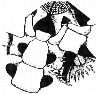
Figure 26. Ophiothrix spiculata .
