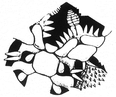
Figure 28. Ophiopholis bakeri .
