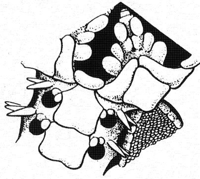
Figure 14. Amphiodia occidentalis .
