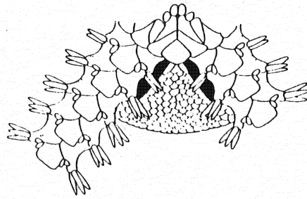
Figure 10. Amphipholis squamata .
