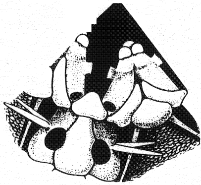
Figure 6. Amphiura diastata .
