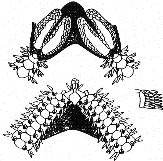
Figure 7. Amphiura arcystata .
