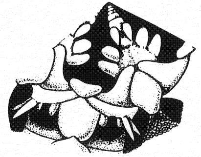
Figure 12. Amphiodia urtica .
