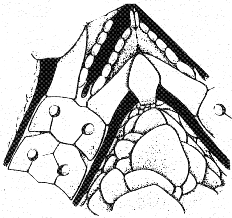
Figure 21. Ophiomusium jolliensis .
