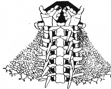
Figure 11. Amphiodia digitata .
