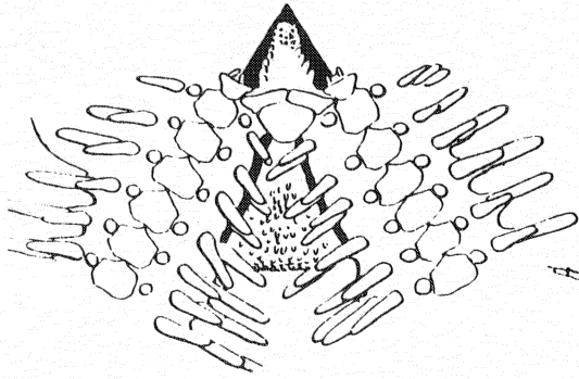
Figure 25. Ophiopteris papillosa .
