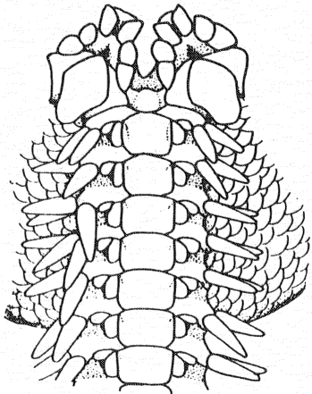
Figure 13. Amphiodia psara .
