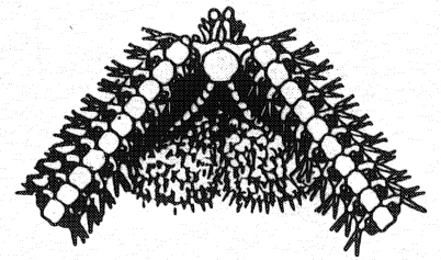
Figure 15. Amphiacantha amphacantha .
