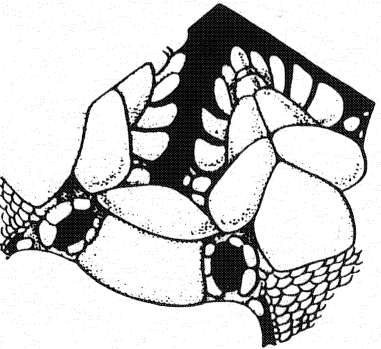
Figure 22. Ophioplocus esmarki .
