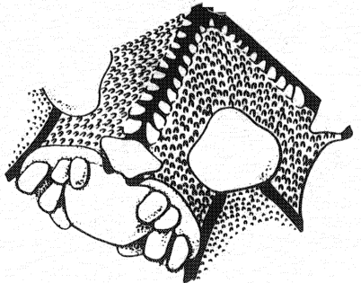
Figure 23. Ophioderma panamense .
