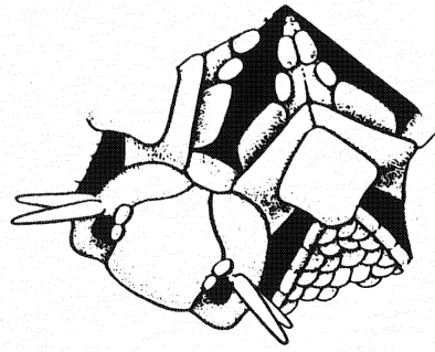
Figure 10. Amphipholis squamata .
