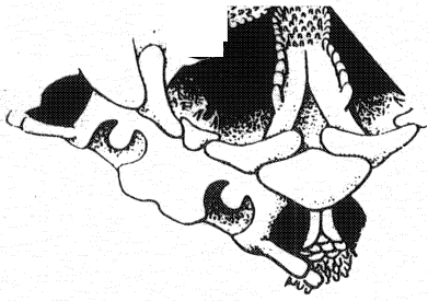
Figure 25. Ophiopteris papillosa .
