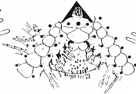
Figure 26. Ophiothrix spiculata .
