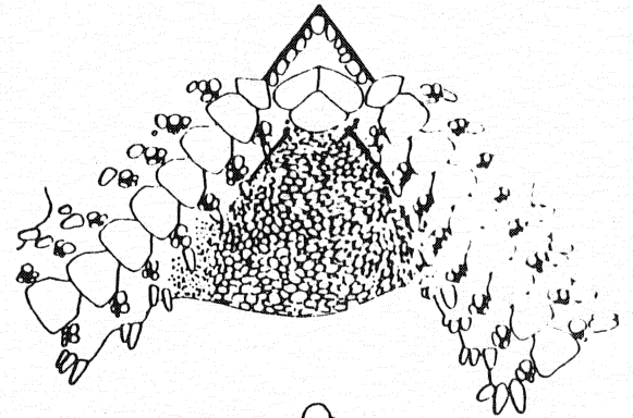
Figure 22. Ophioplocus esmarki .
