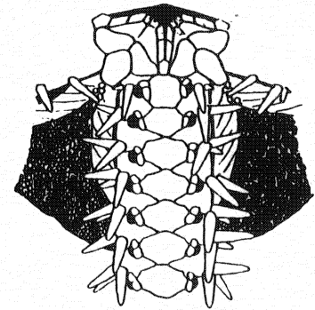
Figure 8. Amphichondrius granulatus .
