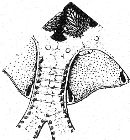
Figure 3. Gorgonocephalus eucnemis .
