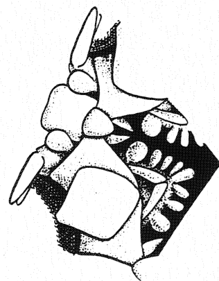
Figure 19. Ophioneis annulata .
