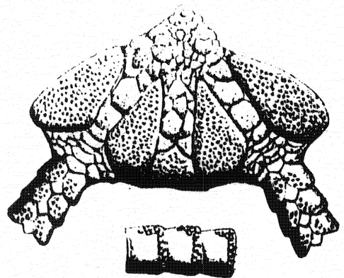
Ophiomusium lymani
