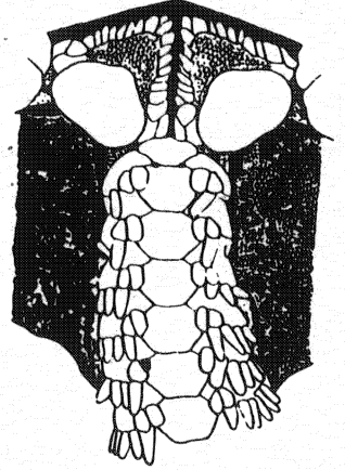
Figure 23. Ophioderma panamense .
