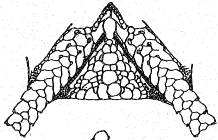
Figure 21. Ophiomusium jolliensis .
