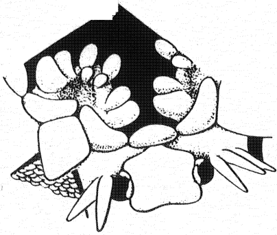
Figure 13. Amphiodia psara .
