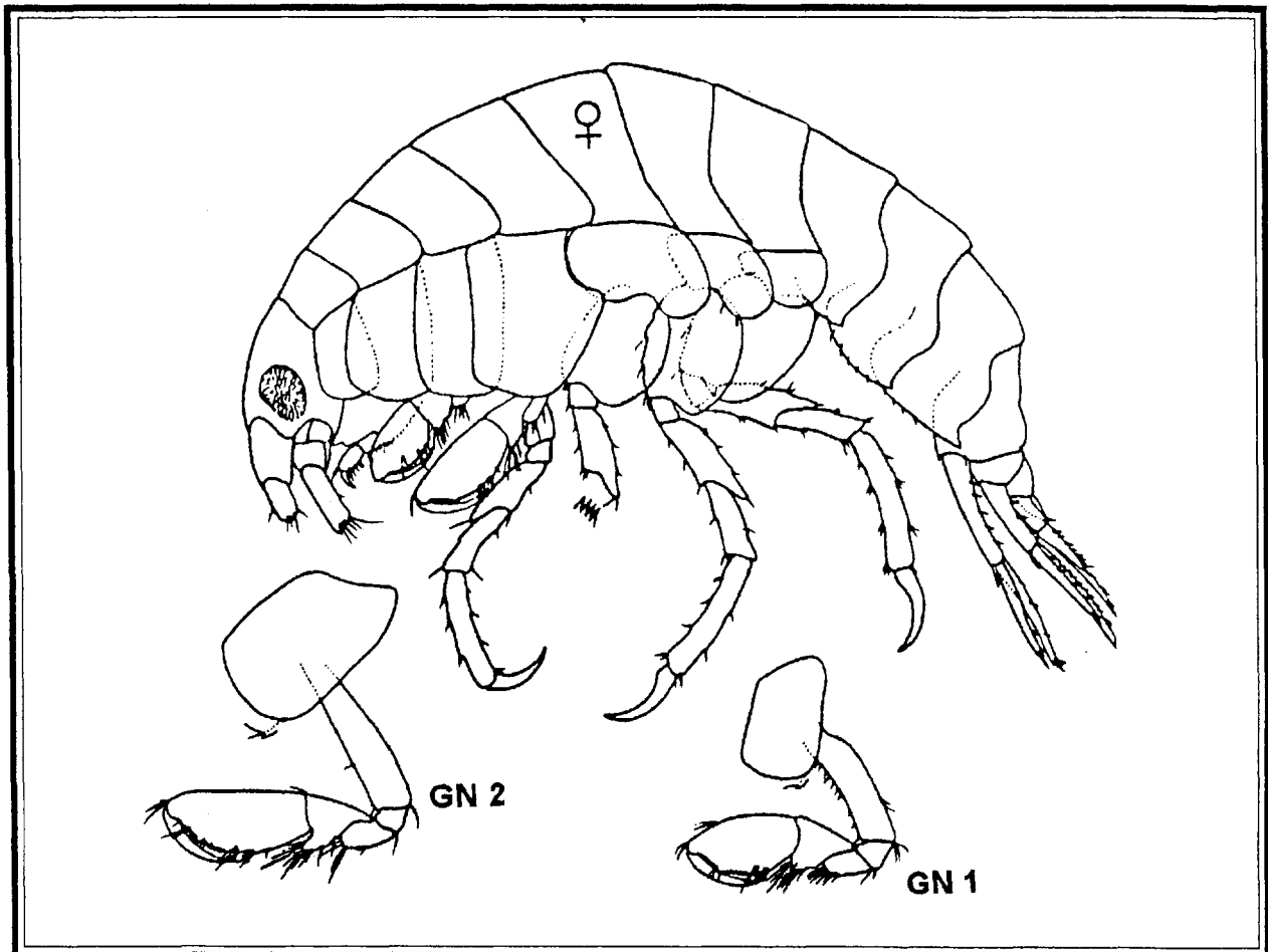
Figure 3.28. Pleusymtes subglaber (from Barnard and Given, 1960).
