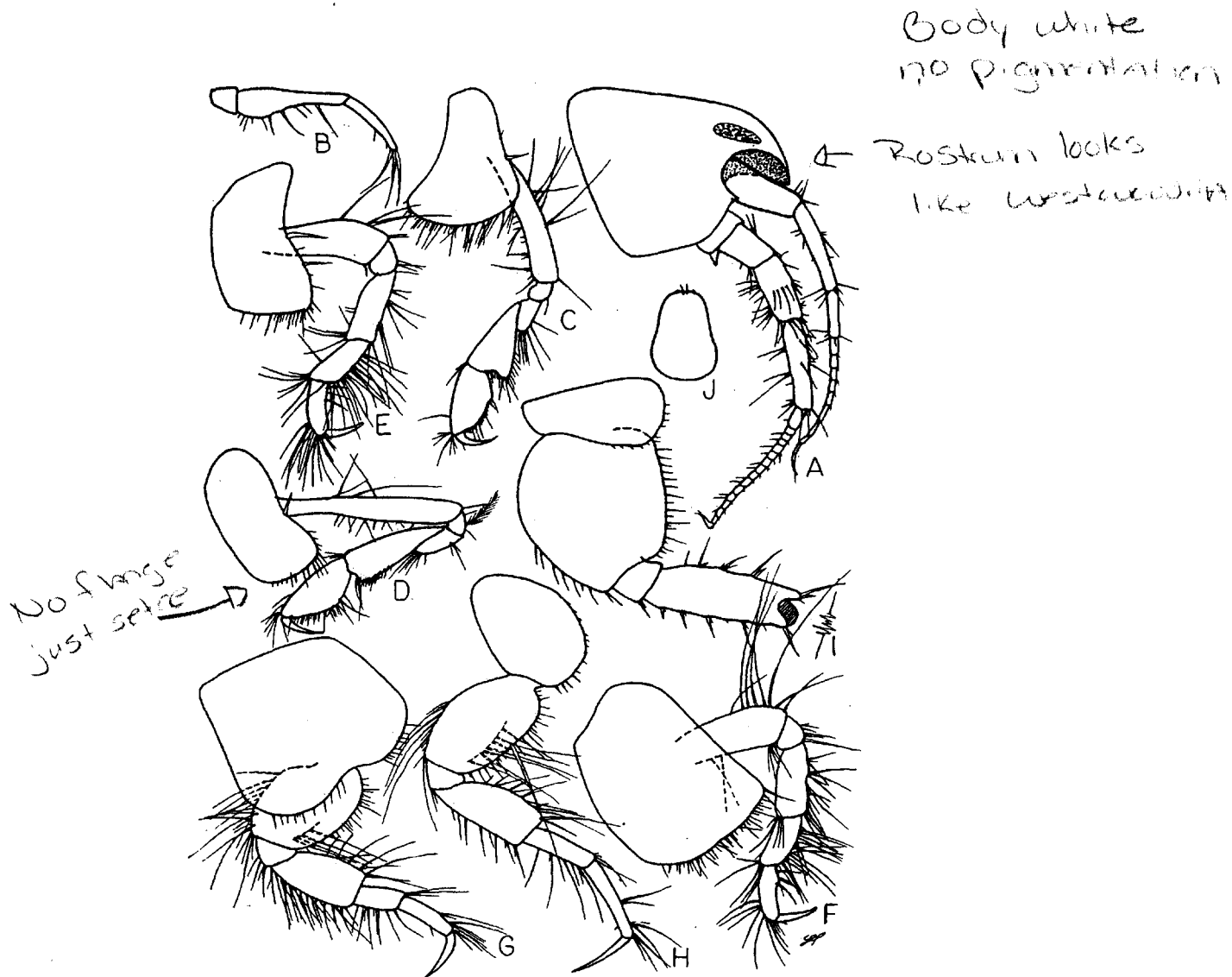
Fig. 2. Bathymedon roquedo , n. sp. ?Male, holotype, 5.5 mm, sta. 3727: A, head; B, mandibular palp; C, D, gnathopods 1, 2; E, F, G, H, I, pereopods 1, 2, 3, 4, 5; J, telson.
