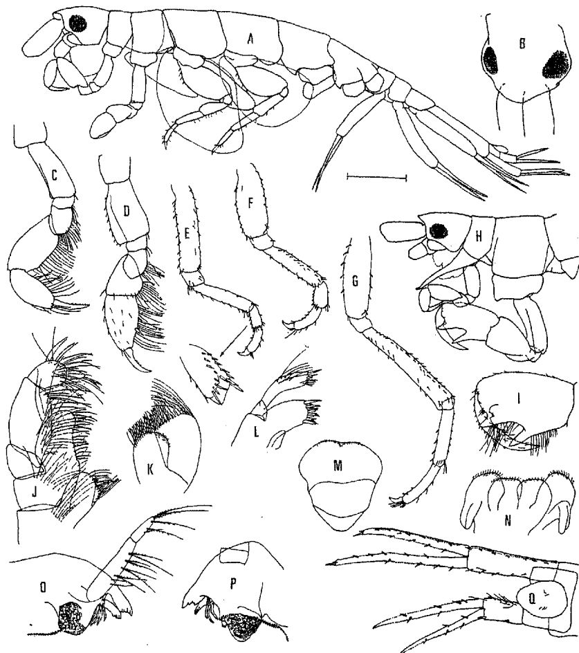
FIG. 15. Dyopodos monacanthus . A, lateral view; B, dorsal view head; C and D, ♀ gnathopods 1 and 2; E-G, pereopods 5-7; H, anterior of ♂; I, ♂ gnathopod 2 propodus; J, maxilliped; K and L, maxilla 2 and 1; M and N, upper and lower lip; O and P, left and right mandible; Q, posterior urosome.
