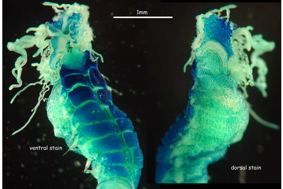
thoracic uncini
