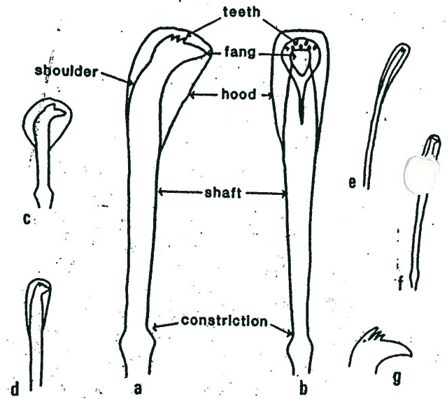
Fig. 1. Structure of the hooded hooks: a - generalised hooded hook, lateral view; b - generalised hooded hook, frontal view; c - typical abdominal hooded hook; d - typical thoracic hooded hook; e - Mediomastus acutus notosetal "hook"; f - M. ambiseta abdominal "spine-like" hook; g - M. thomassini n.sp. abdominal hooded hook.
