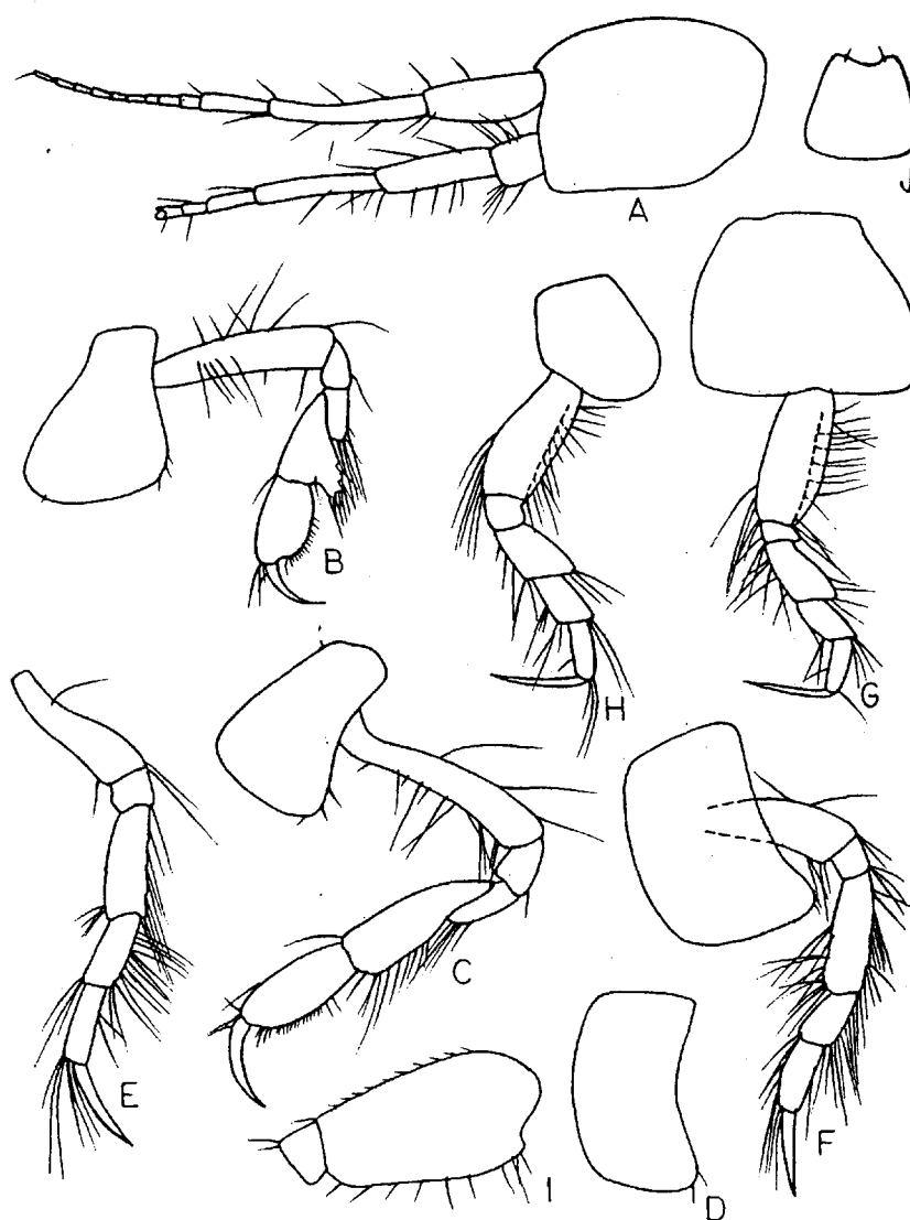
Fig. 1. Bathymedon pumilus , n. sp. Male, 2.5 mm, sta. 4753: A, head; B, C, gnathopods 1, 2; D, coxa 3; E, F, G, H, I, peraeopods 1, 2, 3, 4, 5; J, telson.
